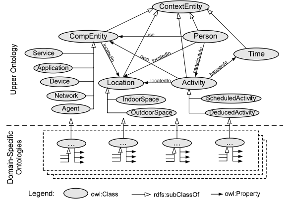
Figure 1. An example of context ontology
