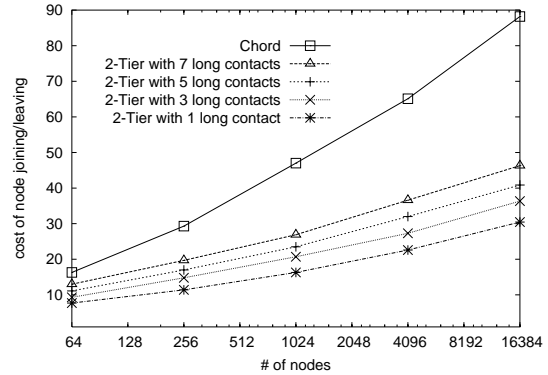
Figure 7. Cost of node joining/leaving
