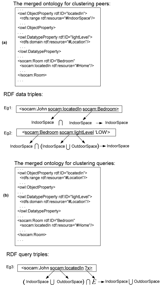
Figure 2. An example of semantic cluster mapping
