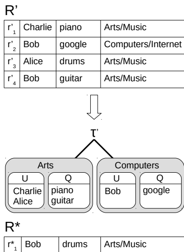
FIGURE 2. Contents of \tau' and R^* when trying to deanonymize R' from the example provided in Table 2.
