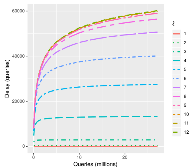
FIGURE 13. Queries delay, as the mean number of other queries that enter the system during the period between the entry and the leave of a given query. Once the categories are full, the output stabilizes.
