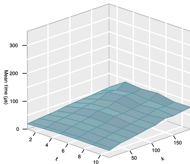
FIGURE 11. Anonymizer mean time per query ( \mu\text{s} ). \ell -value has little effect on required time, k -value has a greater effect.
