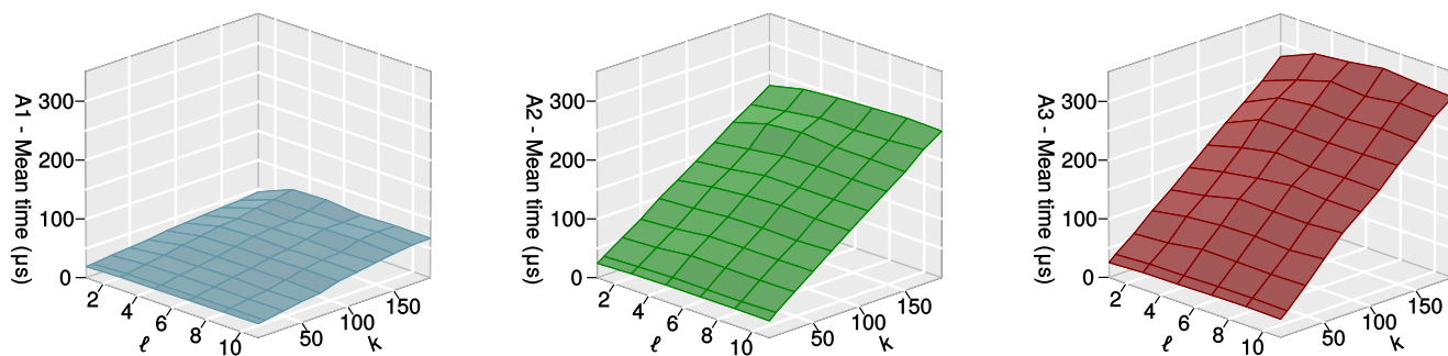
FIGURE 12. De-anonymizer mean time per query ( \mu\text{s} ). First de-anonymizer obtained comparable results to the anonymizer. Second and third de-anonymizers, which are more complex, are also slower and are more affected by increases in k -value.
