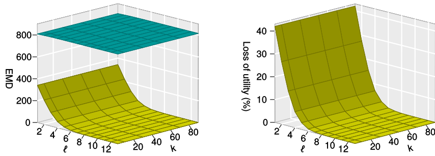
FIGURE 10. (a) Maximum theoretical distance between profiles, constant, and average EMD distances, inversely proportional to \ell . (b) Loss of utility (%), the more levels we use in our anonymizer, the better data utility.
