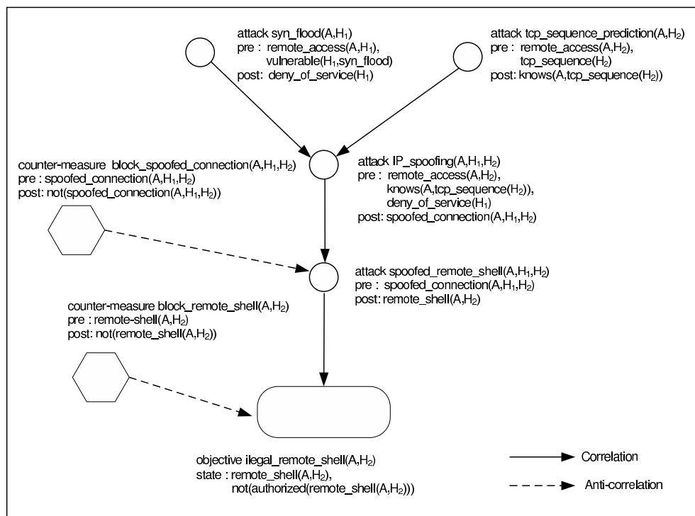
Figure 6.8: Correlation graph for the Mitnick attack scenario.
